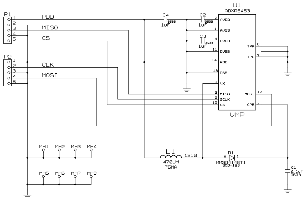
Figure 2. EVAL-ADXRS453Z-V Schematic
