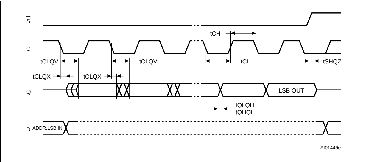
Figure 26. Output timing
