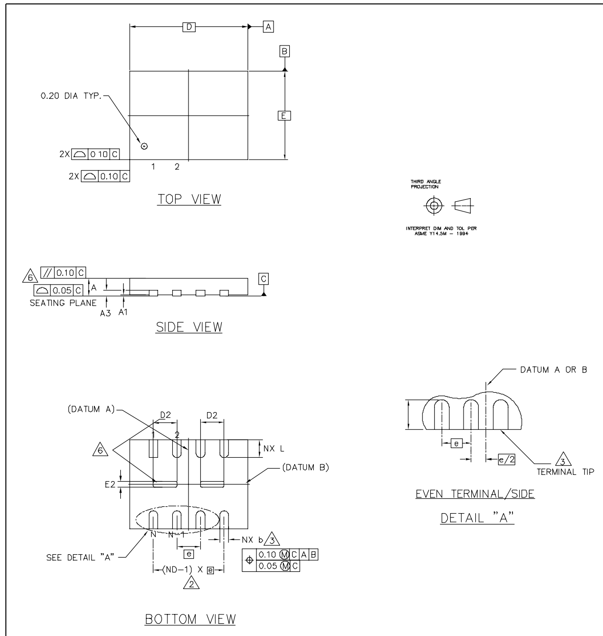
Figure 33. UFDFPN (MLP8) 8-lead ultra thin fine pitch dual flat package no lead, 4X3 mm package mechanical data
