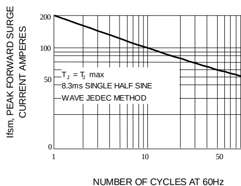
Fig. 6-MAXIMUM NON-REPETITIVE PEAK FORWARD SURGE CURRENT UNIDIRECTIONAL
