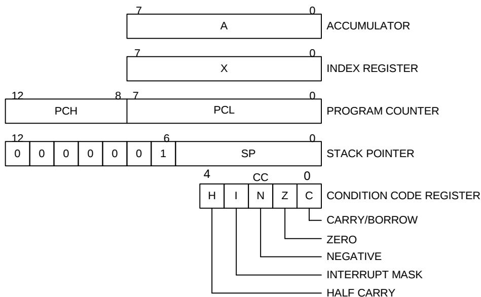
Figure 6. Programming Model
