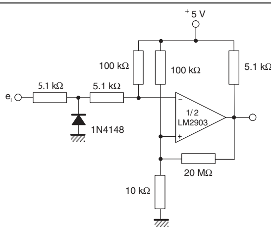
Figure 14. Zero crossing detector (single power supply)
