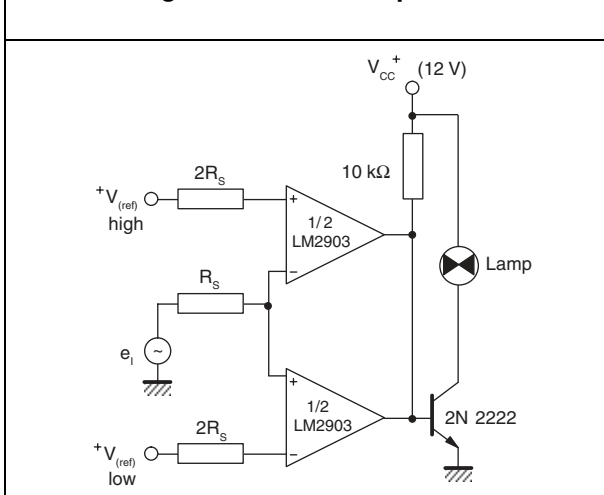
Figure 15. Limit comparator
