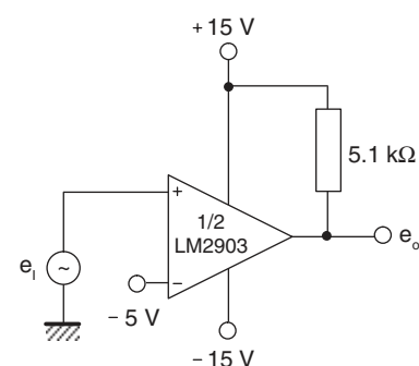
Figure 18. Comparator with a negative reference
