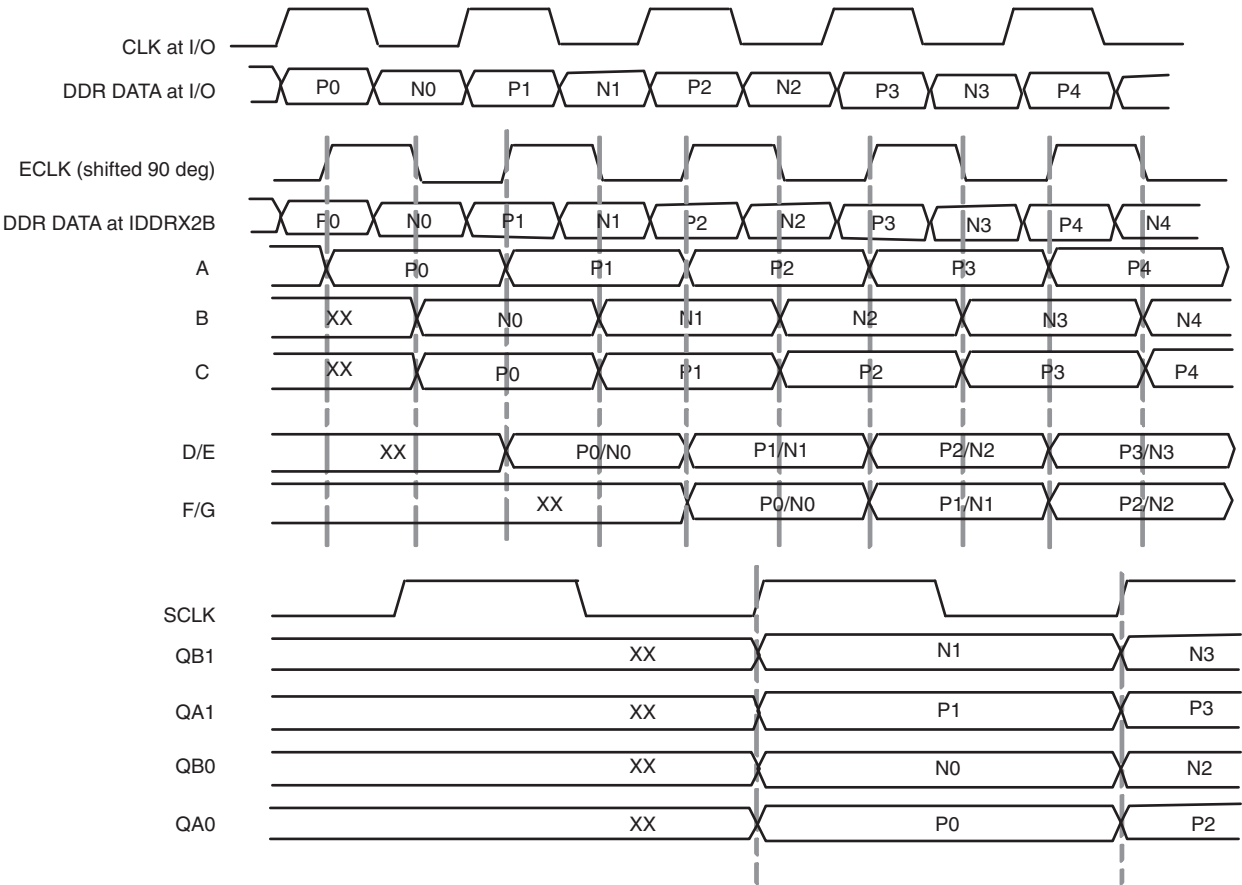
Figure 12-34. IDDRX2B Waveform
