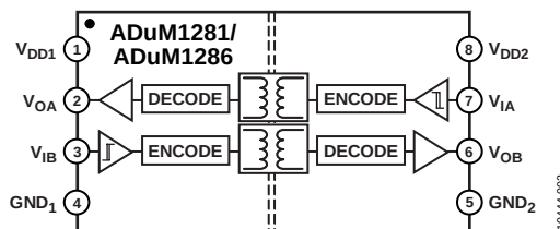
Figure 2. ADuM1281/ADuM1286
