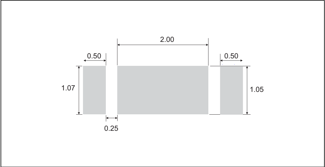
Figure 9. Footprint (dimensions in mm)
