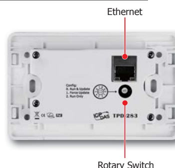
TPD-283 Rear View
