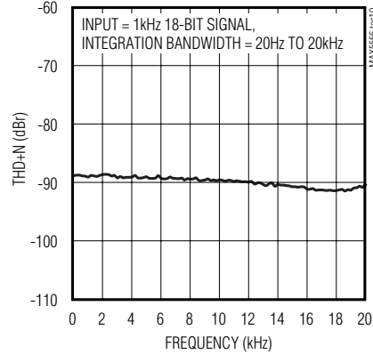
UNWEIGHTED THD+N vs. FREQUENCY
