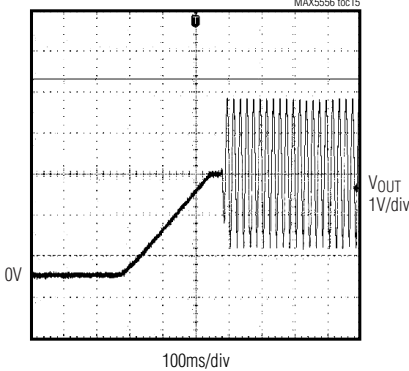
POWER-UP RESPONSE
