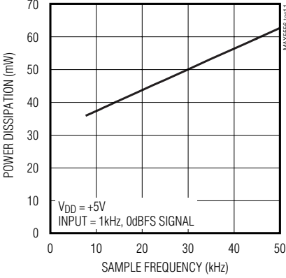
POWER DISSIPATION vs. SAMPLE FREQUENCY
