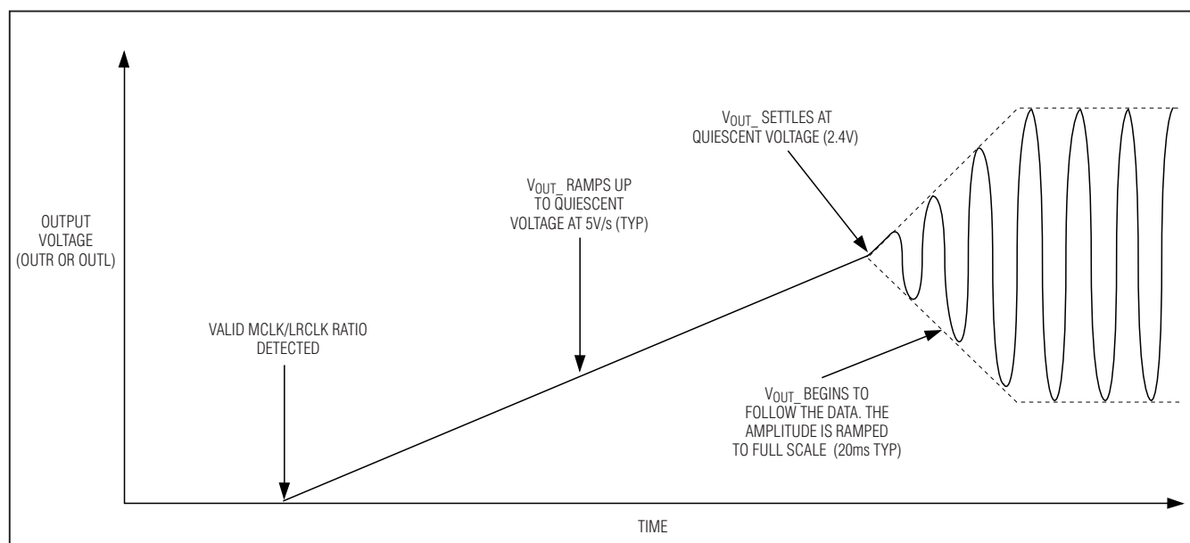
Figure 11. Power-Up Sequence
