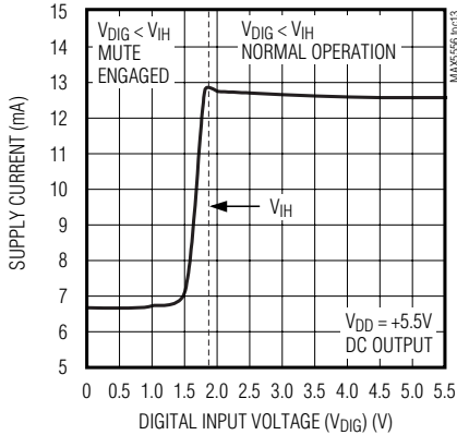
SUPPLY CURRENT vs. DIGITAL INPUT VOLTAGE ( V_{DIG} )
