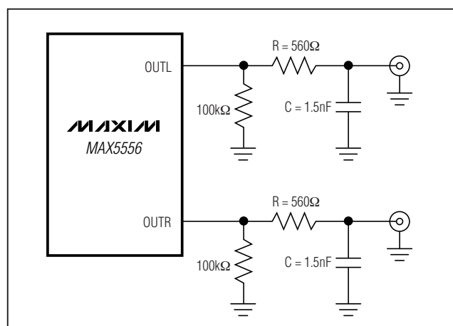
Figure 8. Passive Component Analog Output Filter
