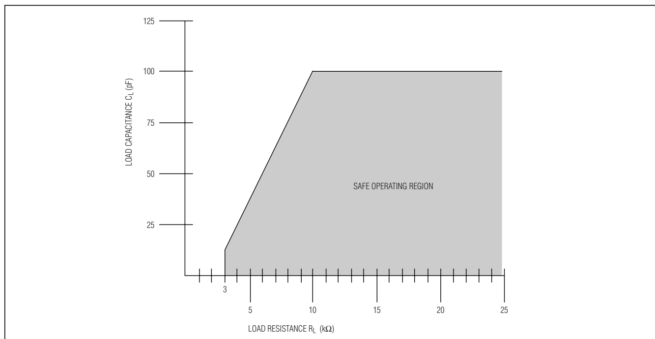
Figure 3. Load-Impedance Operating Region
