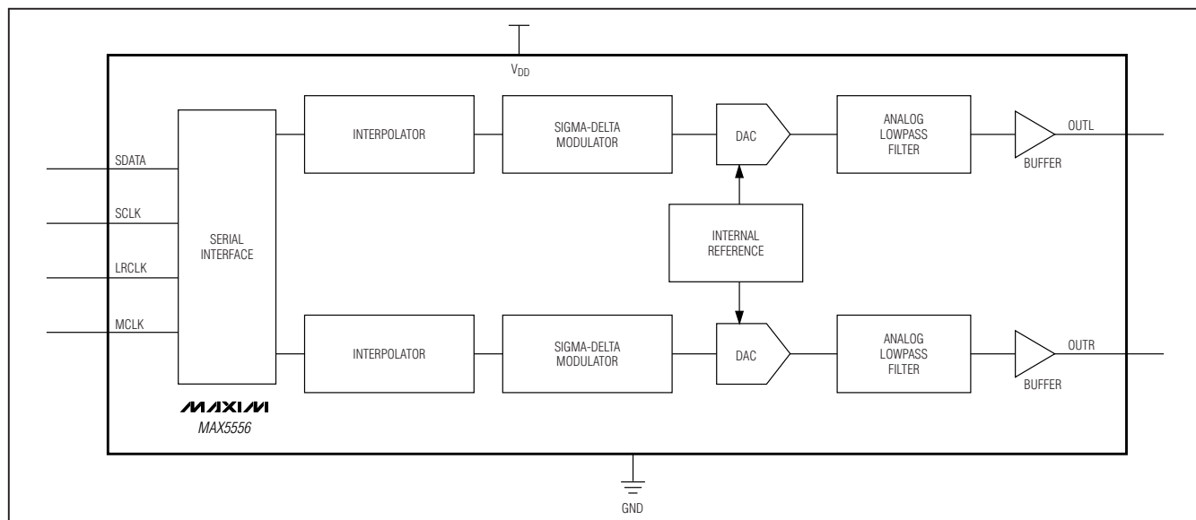
Figure 2. Functional Diagram
