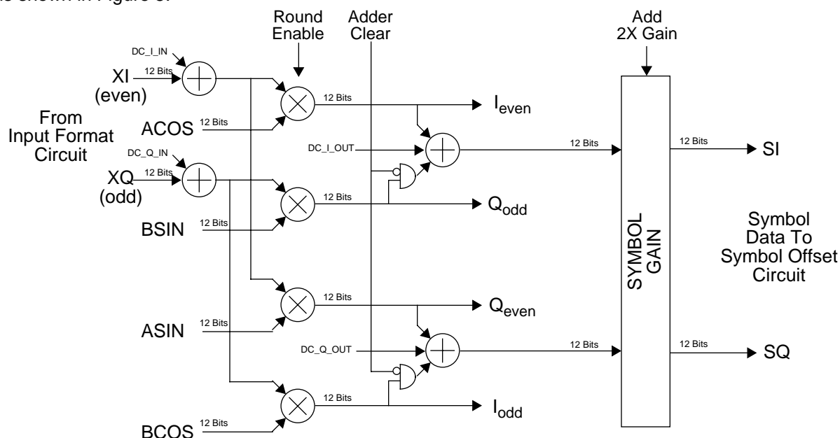
Figure 5. MIXER
