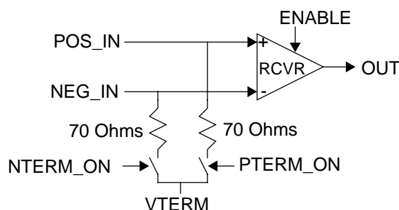
Figure 4. DIFFERENTIAL INPUT
