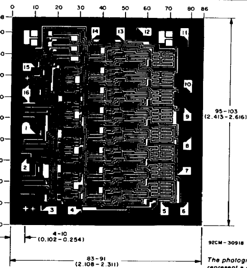
CD4724BH DIMENSIONS AND PAD LAYOUT
