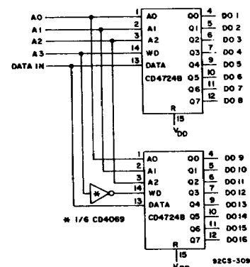
Fig. 14— 1 of 16 decoder/demultiplexer.
