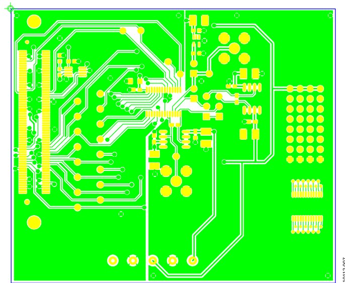
Figure 7. Silkscreen
