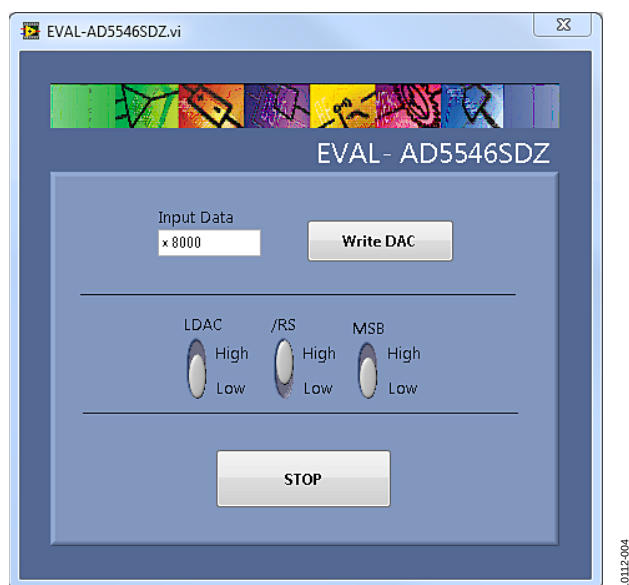
Figure 4. Main Window
