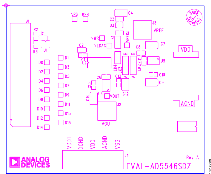
Figure 9. Solder Side
