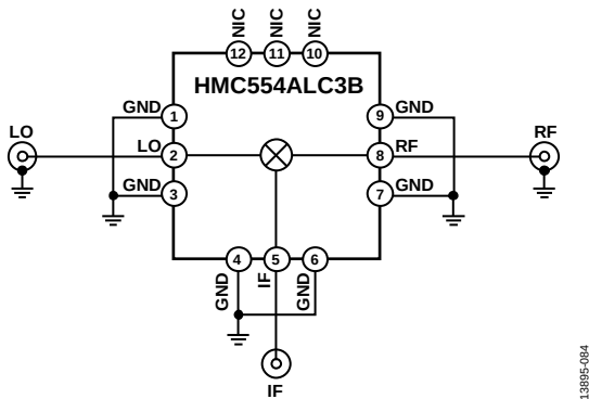
Figure 84. Typical Application Circuit
