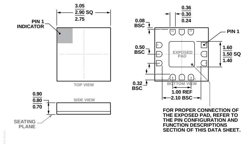
Figure 86. 12-Terminal Ceramic Leadless Chip Carrier (LCC) (E-12-4)
