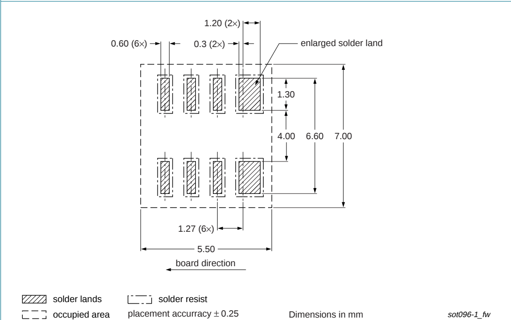
Fig 17. Wave soldering footprint SOT96-1 (SO8)
