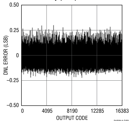
LTC2158-14: Differential Nonlinearity (DNL)
