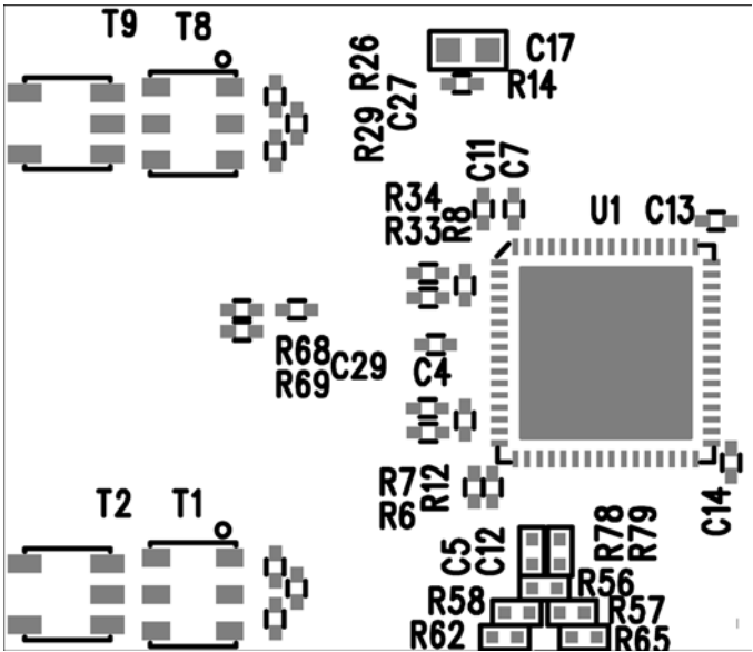
Silkscreen Top
