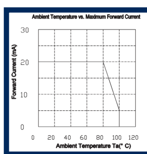
DERATING
