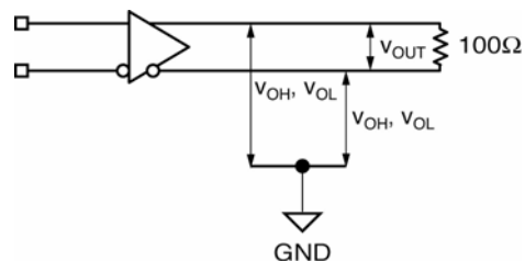
Figure 2a. LVDS Differential Measurement
