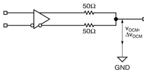
Figure 2b. LVDS Common Mode Measurement
