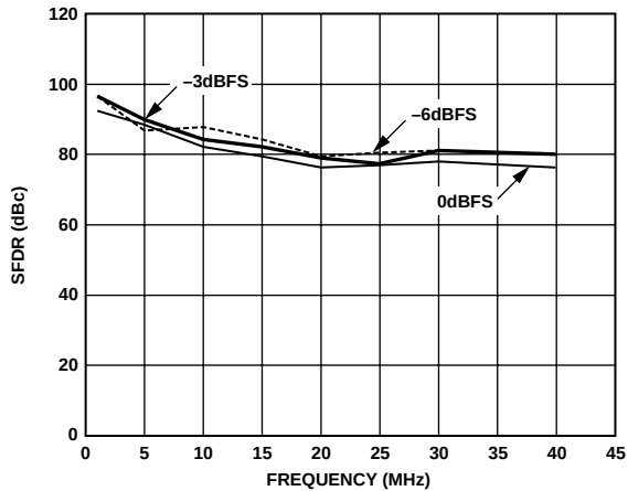
Figure 4. SFDR vs. Frequency, F_{DATA} = 100 MSPS, 4 \times Interpolation
