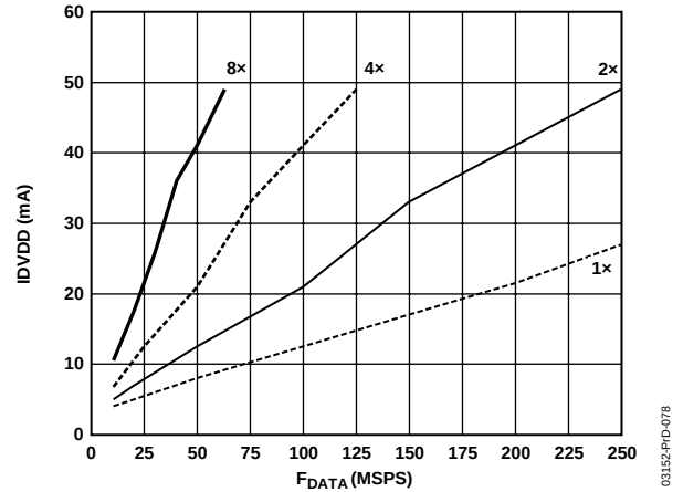
Figure 68. CLKVDD Supply Current vs. Clock Speed and Interpolation Rates
