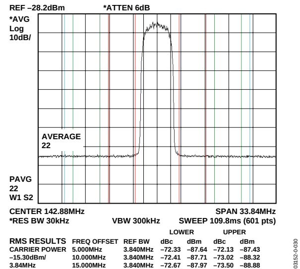
Figure 34. ACLR for Single WCDMA Carrier at 142.88 MHz, F_{DATA} = 61.44 MSPS, 4x Interpolation
