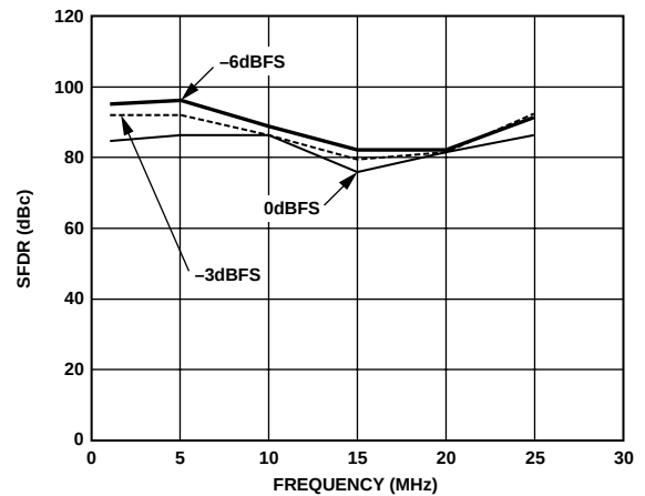
Figure 8. SFDR vs. Frequency, F_{DATA} = 62.5 MSPS, 8 \times Interpolation
