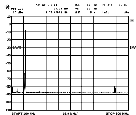
Figure 30. Two Tones around 23 MHz, F_{DATA} = 200 MSPS, 2x Interpolation, Low-Pass Digital Filter Mode
