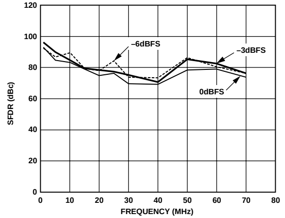
Figure 6. SFDR vs. Frequency, F_{DATA} = 200 MSPS, 2 \times Interpolation
