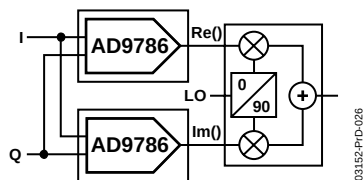
Figure 77. AD9786 Driving Quadrature Modulator
