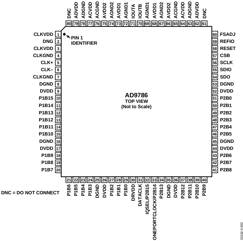
Figure 2. Pin Configuration
