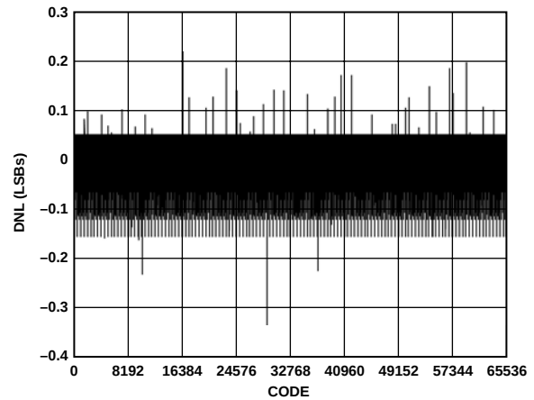
Figure 24. Typical DNL
