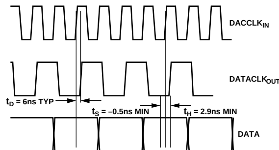
Figure 48. Data Timing, 2 \times Interpolation, DCLKPOL = 1
