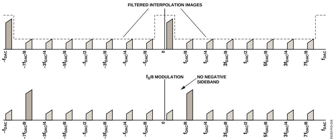
Figure 63. Complex Modulation
