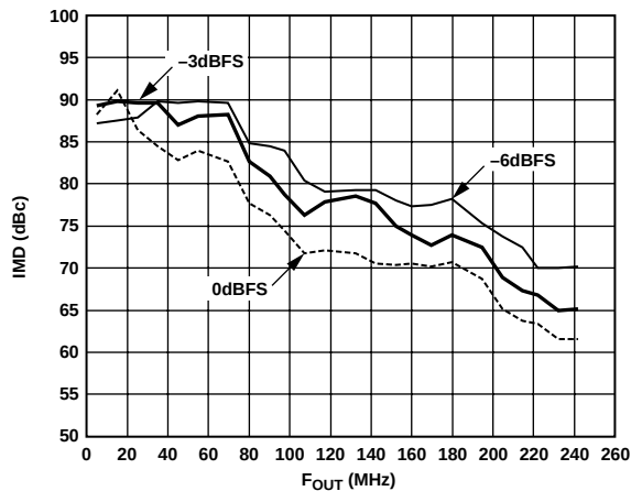
Figure 21. Third Order IMD vs. Frequency, F_{DATA} = 62.5 MSPS, 8× Interpolation
