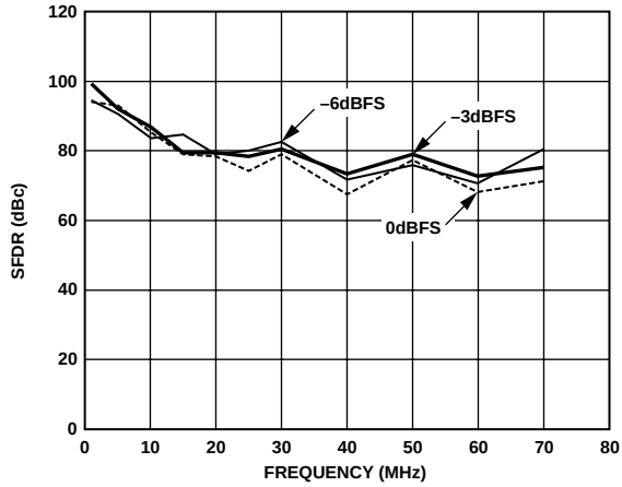
Figure 3. SFDR vs. Frequency, F_{DATA} = 200 MSPS, 1 \times Interpolation
