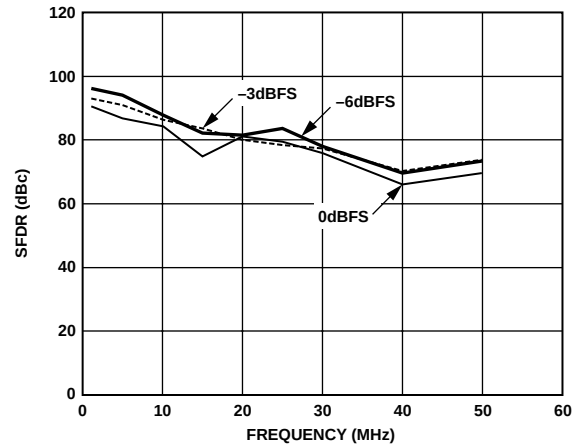
Figure 7. SFDR vs. Frequency, F_{DATA} = 125 MSPS, 4 \times Interpolation
