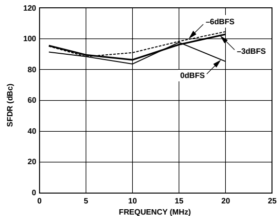
Figure 13. Out of Band SFDR, F_{DATA} = 50 MSPS, 8 \times Interpolation
