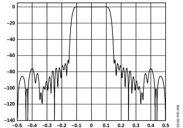
Figure 42. \times 4 Interpolation Filter Response
