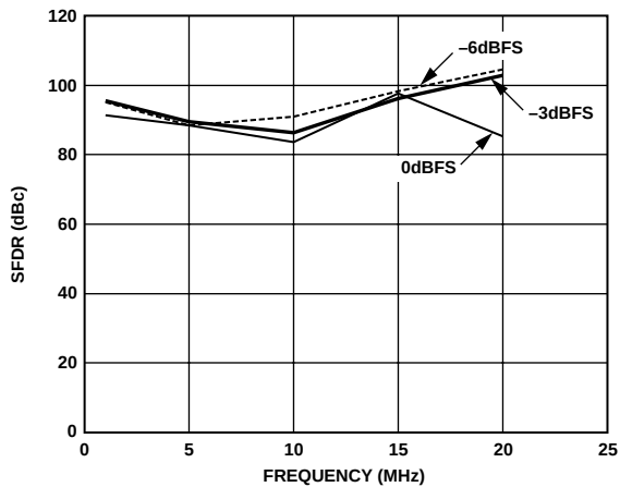
Figure 5. SFDR vs. Frequency, F_{DATA} = 50 MSPS, 8 \times Interpolation
