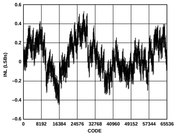
Figure 22. Typical INL
