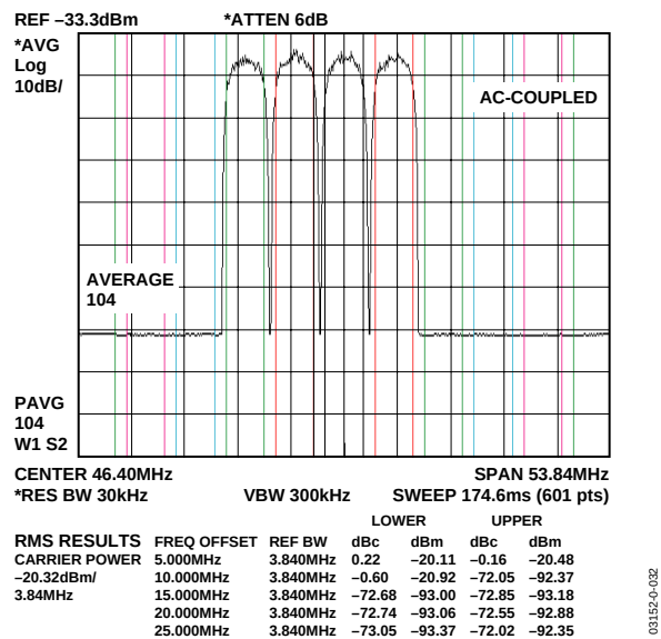
Figure 35. ACLR for Four-Carrier WCDMA Signal Near 50 MHz, F_{DATA} = 61.44 MSPS, 4x Interpolation
