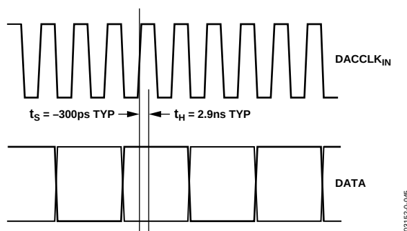
Figure 45. Data Timing, 1× Interpolation, DCLKPOL = 1
