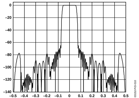
Figure 43. \times 8 Interpolation Filter Response
