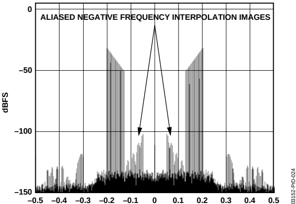
Figure 72. Negative Frequency Aliasing Distortion
