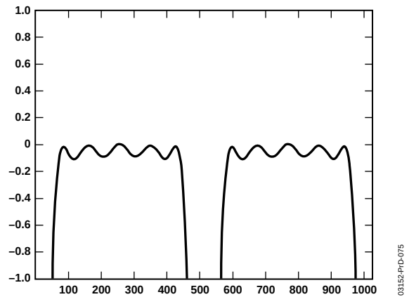
Figure 75. Hilbert Transform Ripple
