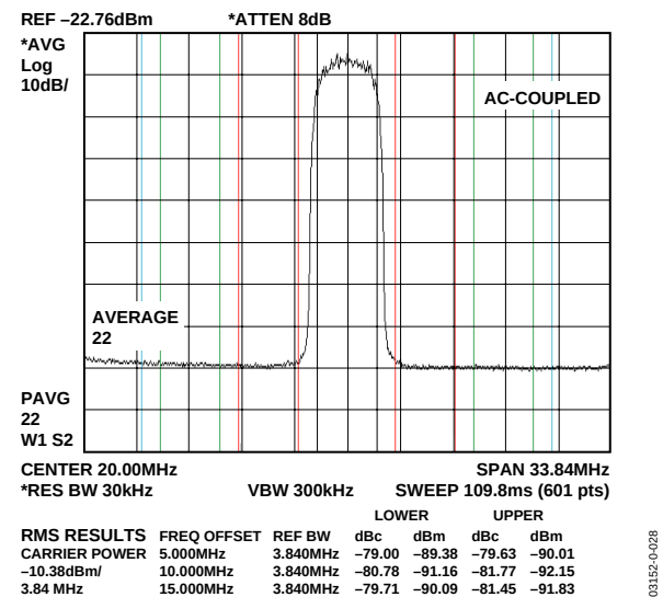
Figure 33. ACLR for Single WCDMA Carrier at 20 MHz, F_{DATA} = 61.44 MSPS, 4x Interpolation
