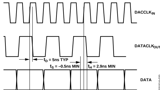
Figure 47. Data Timing, 2 \times Interpolation, DCLKPOL = 0
