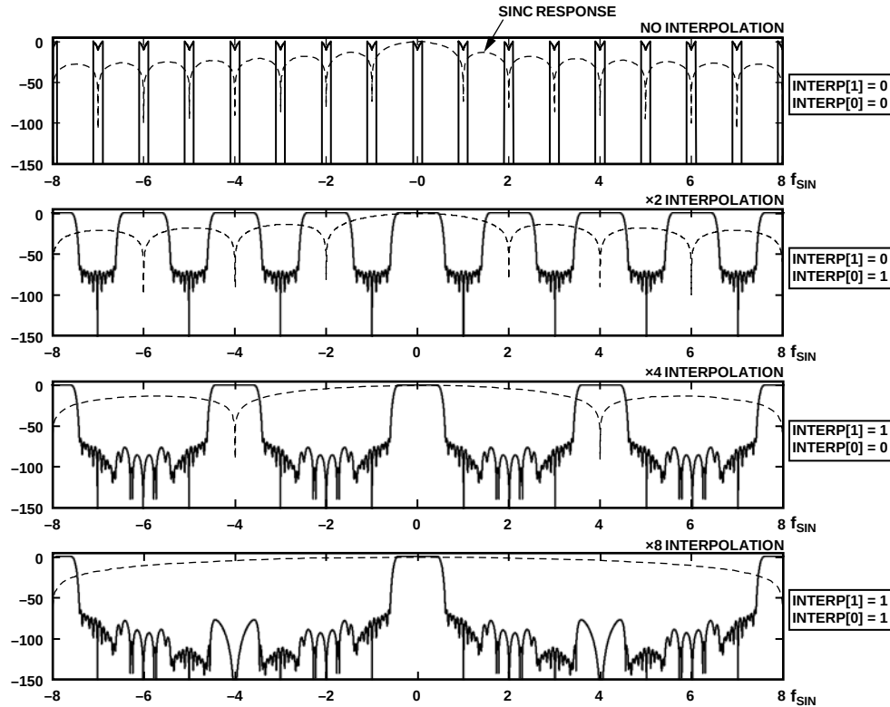
Figure 57. Interpolation Modes
