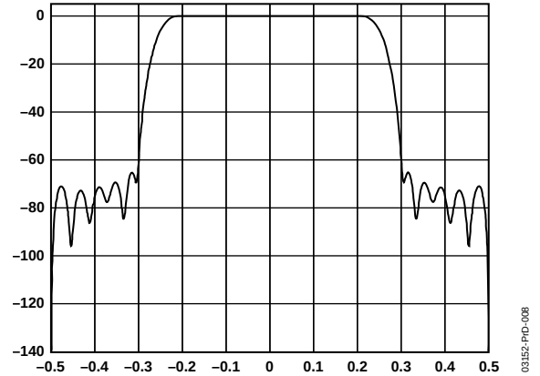
Figure 41. \times 2 Interpolation Filter Response
