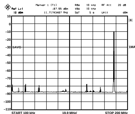
Figure 31. Two Tones around 177 MHz, F_{DATA} = 200 MSPS, 2x Interpolation, High-Pass Digital Filter Mode
