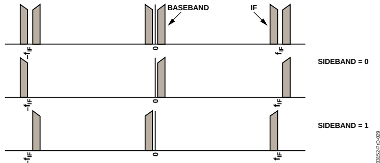
Figure 80. IF Quadrature Modulation of Real and Complex Baseband Signals
