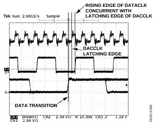
Figure 54. DATAADJ = 0000
