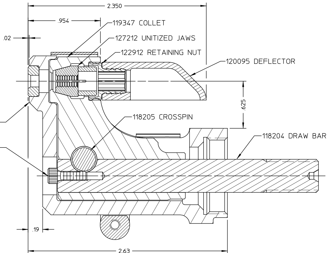
127209 ANVIL ASSEMBLY
