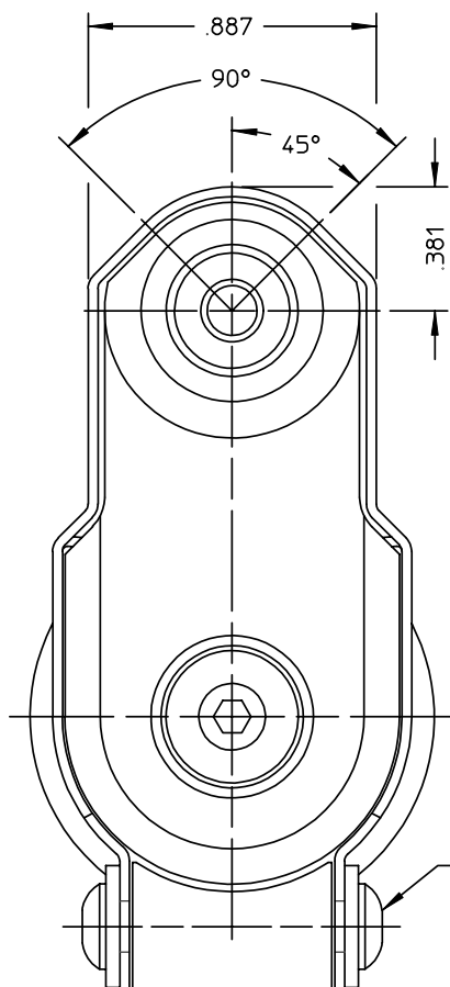
125662 GUARD KIT
