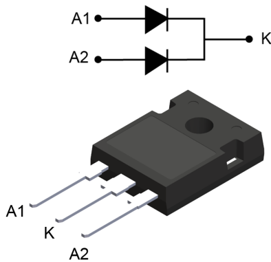
TO-247
