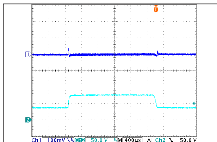
Figure 6: Output voltage response to step-change in input voltage (1000 V/ms). Load cap: 100 μF, electrolytic output capacitance. Ch 1: V out (100 mV/div), Ch 2: V in (50 V/div).
