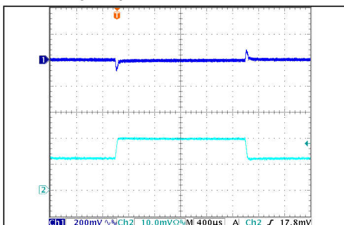
Figure 5: Output voltage response to step-change in load current (50 % -75 % -50 % of I out (max); dI/dt = 0.1 A/μs). Load cap: 100 μF electrolytic capacitor. Ch 1: V out (200 mV/div), Ch 2: I out (10 A/div).
