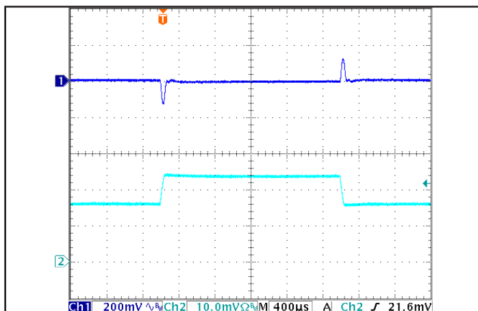
Figure 5: Output voltage response to step-change in load current (50 % -75 % -50 % of I out (max); dI/dt = 0.1 A/μs). Load cap: 100 μF electrolytic capacitor. Ch 1: V out (200 mV/div), Ch 2: I out (5 A/div).
