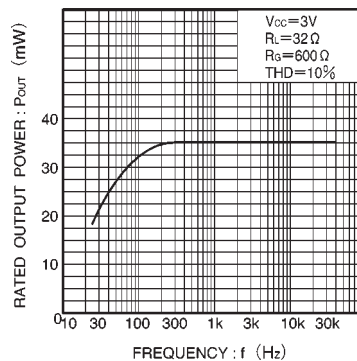
Fig. 6 Rated output power vs. frequency
