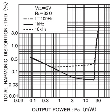
Fig. 4 Distortion vs. output power
