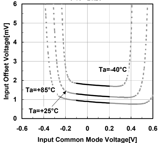
Input Offset Voltage vs. Input Common Mode Voltage V+/V- = \pm 1.2V
