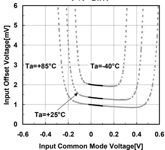
Input Offset Voltage vs. Input Common Mode Voltage V+/V- = \pm 1.1V
