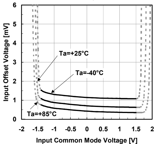
Input Offset Voltage vs. Input Common Mode Voltage V+/V- = \pm 2.5V
