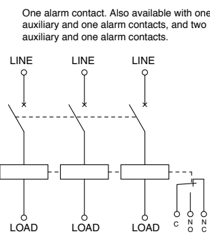
NC1V-3121 (With alarm contact)
