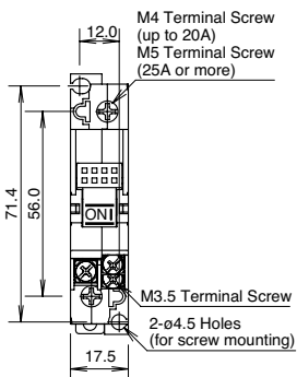
NC1V-1111 (Auxiliary Contact) NC1V-1121 (Alarm Contact)
