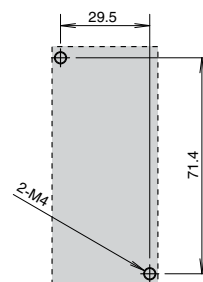
Mounting Hole Layout (M4 Mounting Screws)
