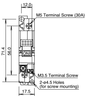
NC1V-1500 (Relay Trip)
