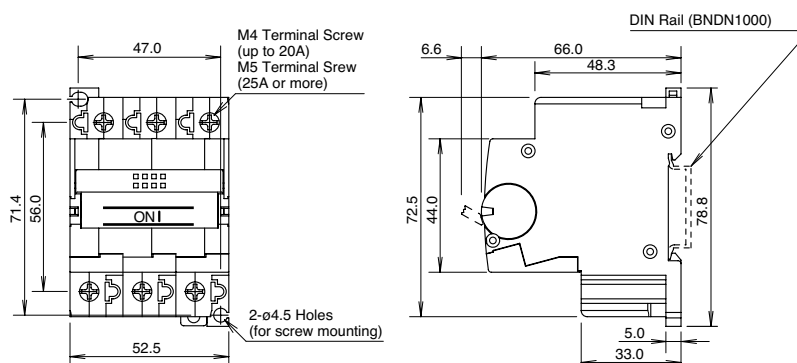
Mounting Hole Layout (M4 Mounting Screws)
