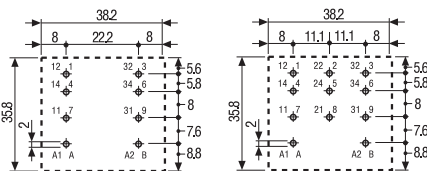
62.22 Copper side view 62.23 Copper side view
