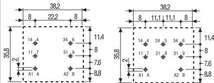
62.22-0300 Copper side view 62.23-0300 Copper side view
