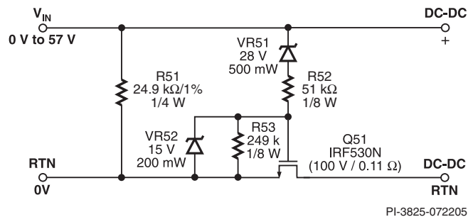
Figure 1. PoE Class 0 Interface Circuit Using a MOSFET Pass-Switch.
