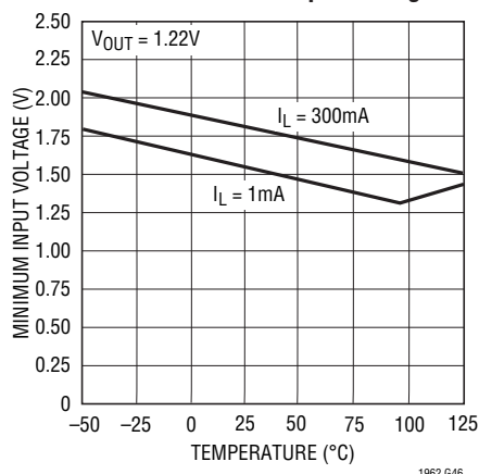
LT1962 Minimum Input Voltage
