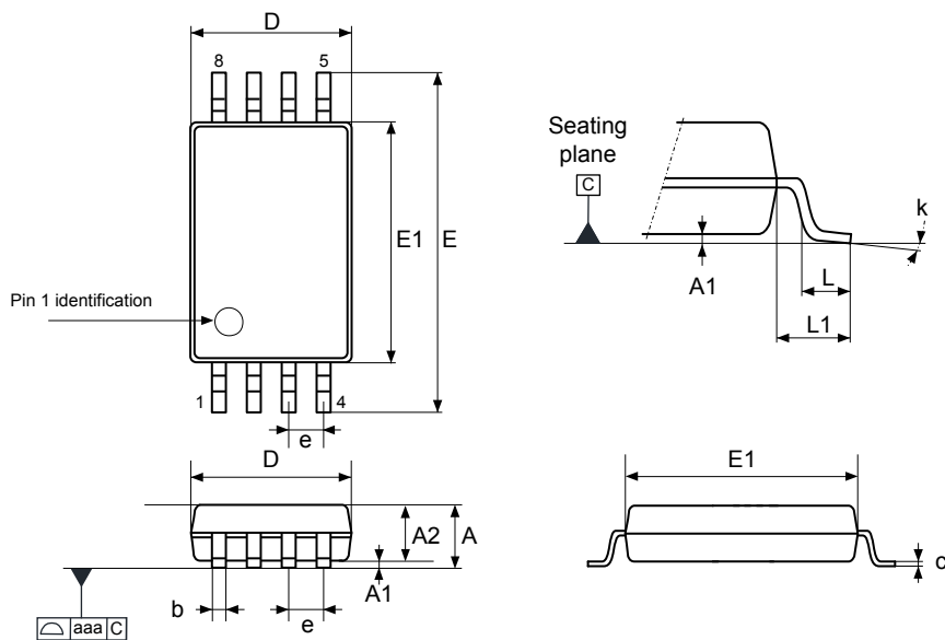
Figure 24. TSSOP8 – Outline
