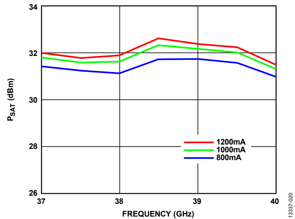
Figure 20. P_{SAT} vs. Frequency for Various Supply Currents
