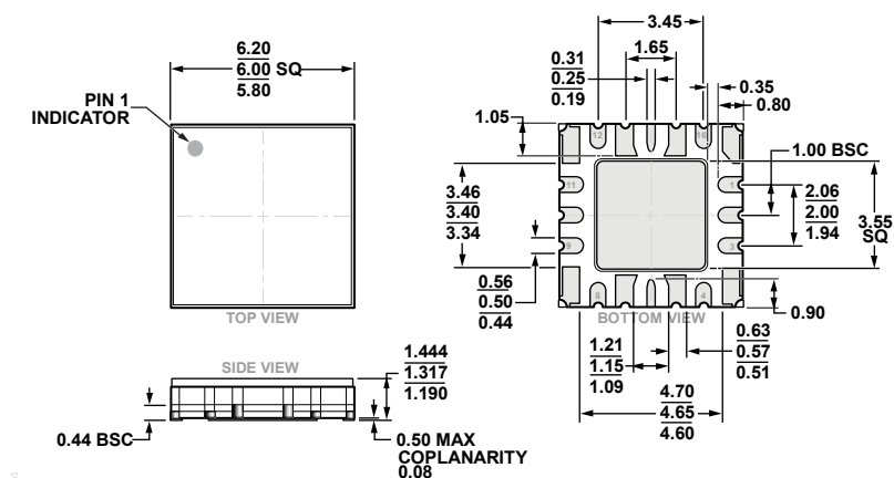
Figure 36. 16-Terminal Ceramic Leadless Chip with Heat Sink [LCC_HS] (EP-16-2)
