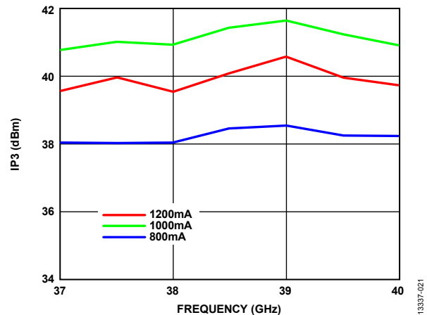
Figure 21. Output IP_3 vs. Frequency for Various Supply Currents, P_{OUT}/Tone = 20\text{ dBm}
