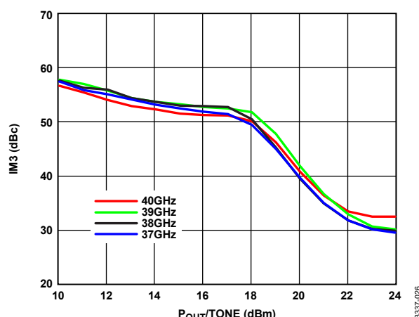
Figure 26. Output IM3 at V_{DD} = 6 V vs. P_{OUT/TONE}
