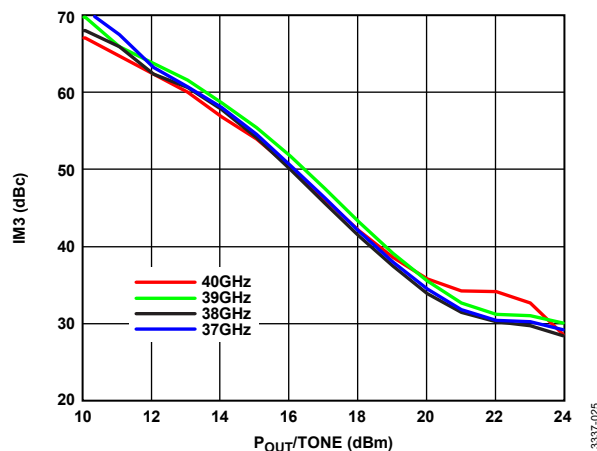
Figure 25. Output IM3 at V_{DD} = 5 V vs. P_{OUT/TONE}
