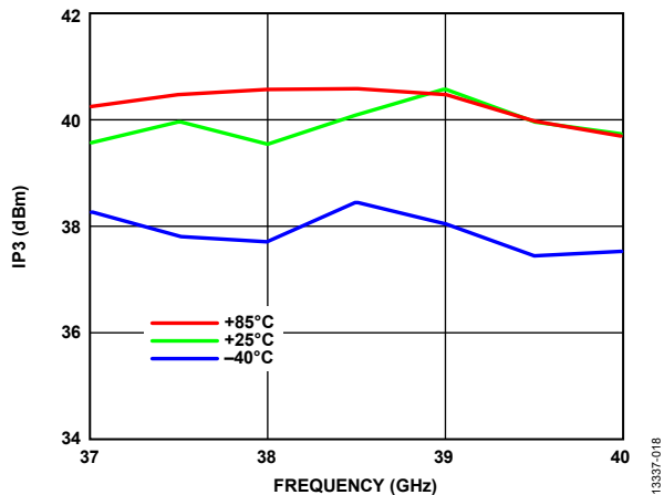
Figure 18. Output IP_3 vs. Frequency for Various Temperatures, P_{OUT}/Tone = 20\text{ dBm}
