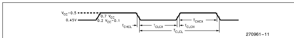
Figure 10. Clock Signal Waveform for I_{CC} Tests in Active and Idle Modes. T_{CCH} = T_{CHCL} = 5 \text{ ns}.
