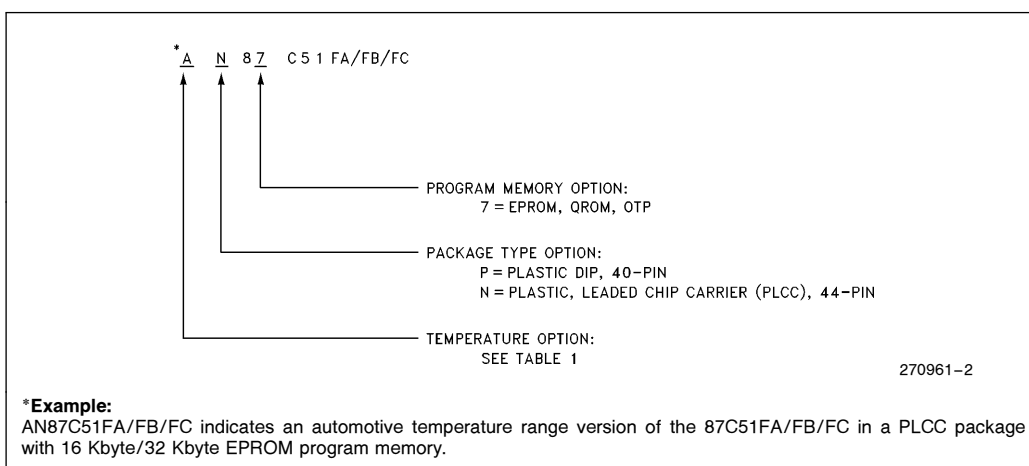
Figure 2. Package Options
