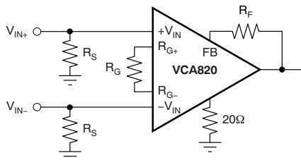
Figure 1. Differential Equalizer
