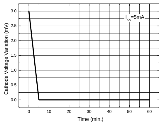
Figure 8. Cathode Voltage Variation vs. Time
