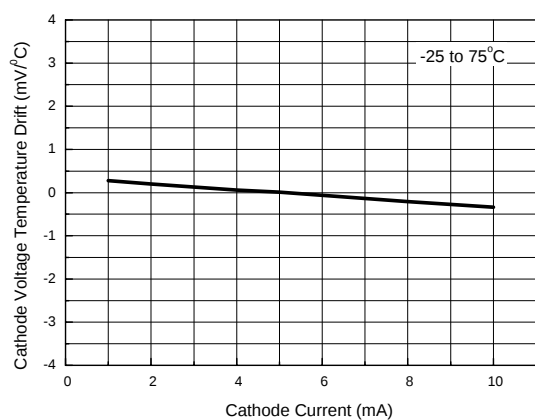
Figure 6. Cathode Voltage Temperature Drift vs. Cathode Current
