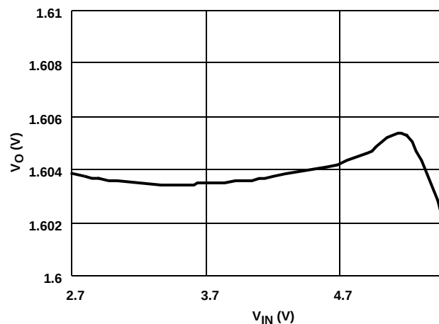
FIGURE 8. LINE REGULATION ( I_O = 1A )
