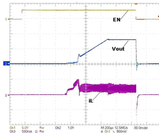
FIGURE 10. SOFT-START
