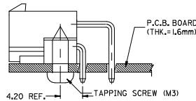
RECOMMENDED INSTALLATION PATTERN
