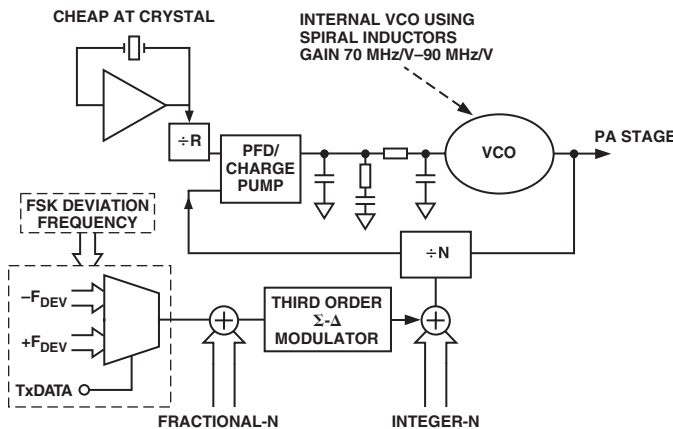
Figure 13. FSK Implementation
