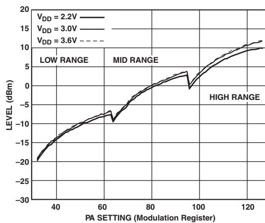
TPC 11. PA Output Programmability, T A = 25°C
