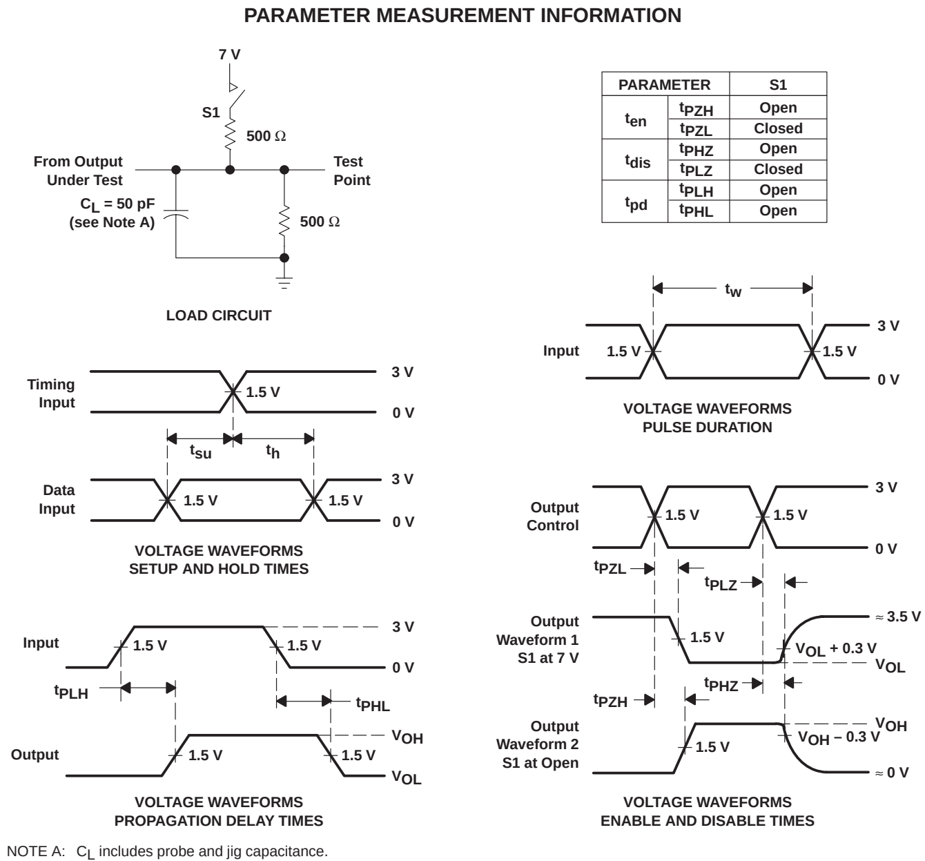
Figure 3. Load Circuit and Voltage Waveforms
