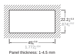
Panel cutout dimensions
