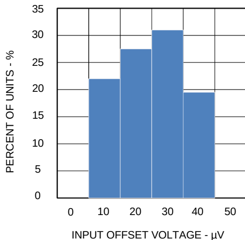
Input Offset Voltage Histogram
