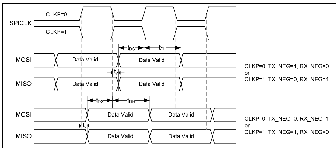
Figure 8-3 SPI Slave timing
