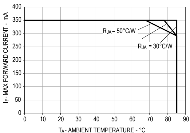
Figure 5. Maximum forward current vs. ambient temperature for AlInGaP Derated based on T_{JMAX} = 110^{\circ}\text{C} , R_{\theta JA} = 30^{\circ}\text{C/W} / 40^{\circ}\text{C/W} and 50^{\circ}\text{C/W}
