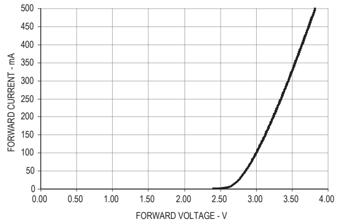
Figure 8. Forward Current vs Forward Voltage for InGaN
