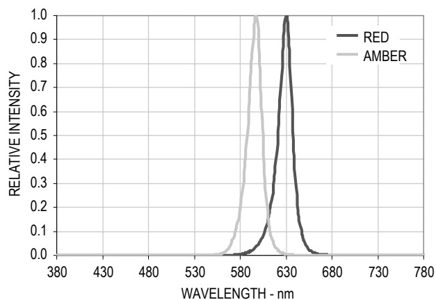
Figure 1. Relative Intensity vs. Wavelength for AlInGaP
