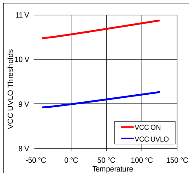
Figure 14: Undervoltage Lockout vs. Temperature
