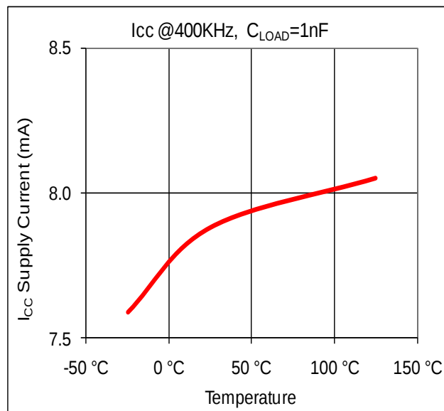
Figure 16: Icc Supply Current @1nF Load vs. Temperature
