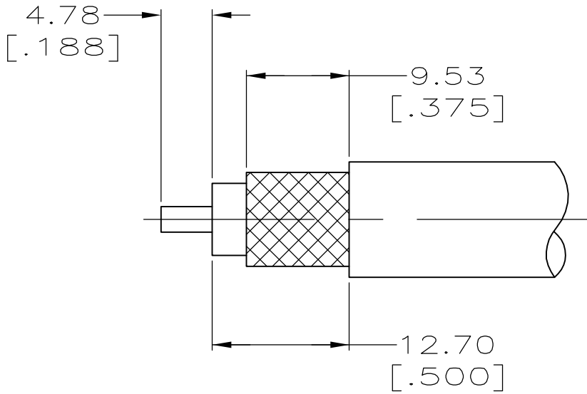
VIEW Y RECOMMENDED STRIP LENGTH SCALE 2:1
