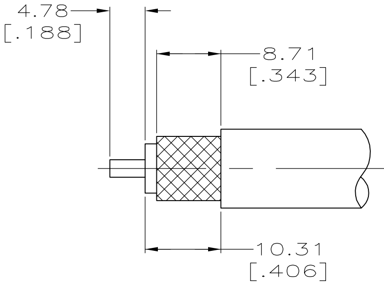
VIEW Z RECOMMENDED STRIP LENGTH SCALE 2:1
