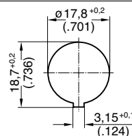
Panel cutout
