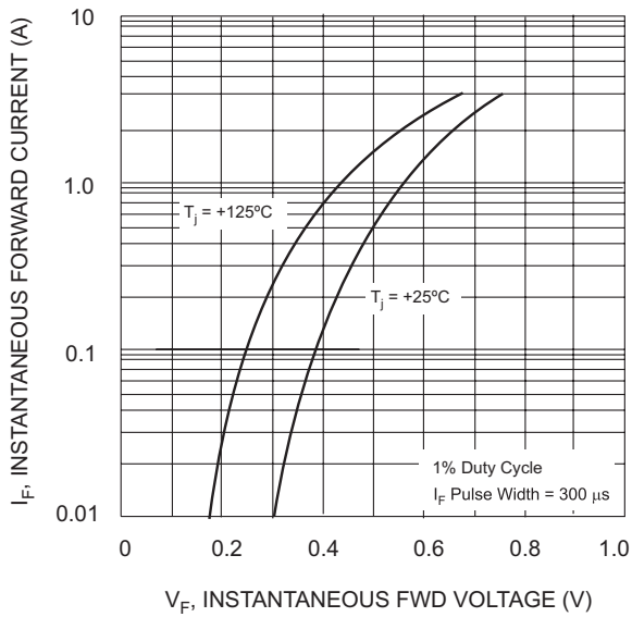
V_F , INSTANTANEOUS FWD VOLTAGE (V) Fig. 3 Typ. Forward Characteristics - SB150 thru SB160
