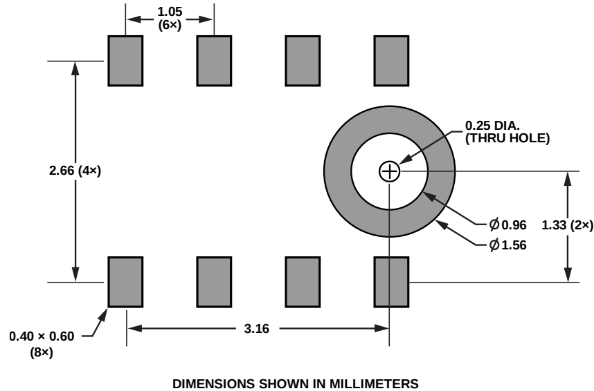
Figure 14. Suggested PCB Land Pattern Layout
