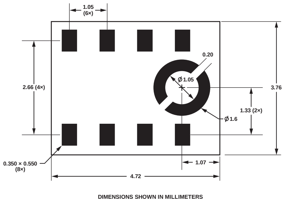
Figure 15. Suggested Solder Paste Stencil Pattern Layout
