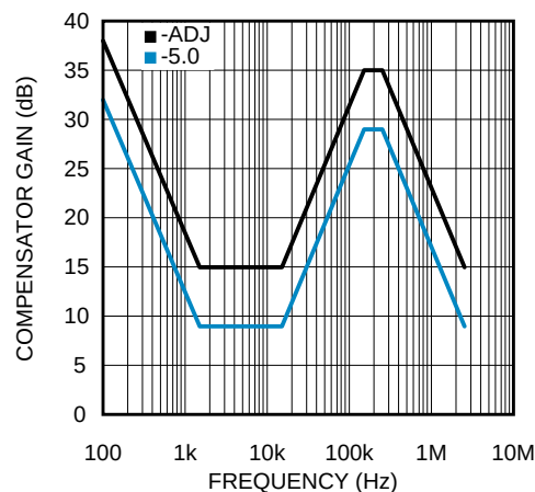
Figure 11. Compensator Gain
