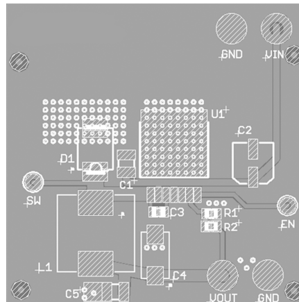
Figure 18. LM22678 Layout Example
