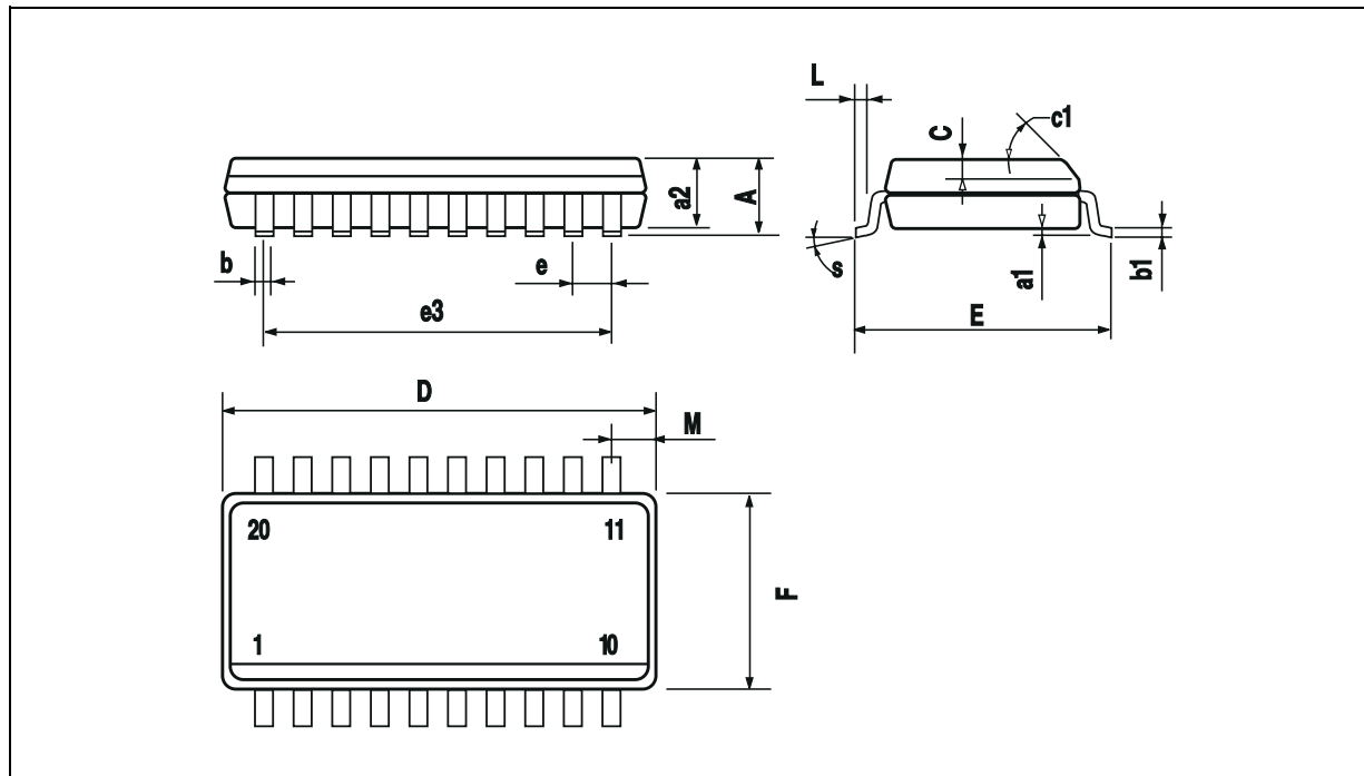
Figure 11. 20-Pin Package
