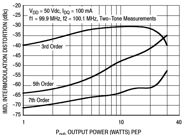
Figure 29. Intermodulation Distortion Products versus Output Power — 100 MHz
