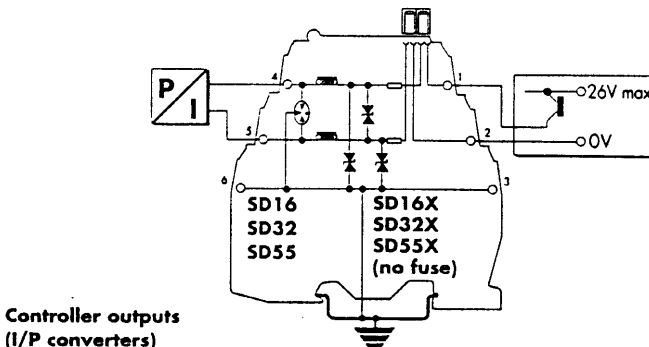
Slidewire displacement transducers
