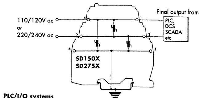
PLC/I/O systems
