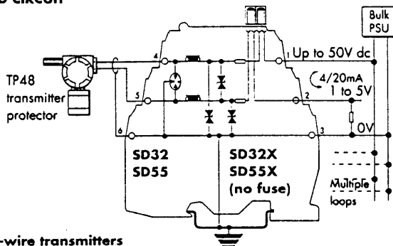
2-wire transmitters
