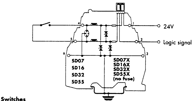
Switches
