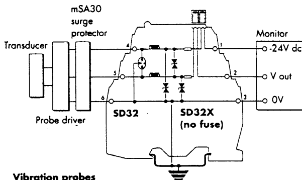
Vibration probes
